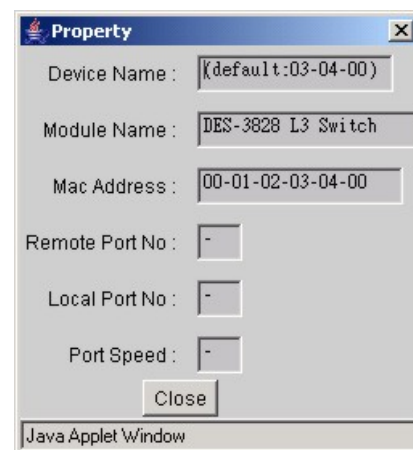
Figure 6- 43. Property window
