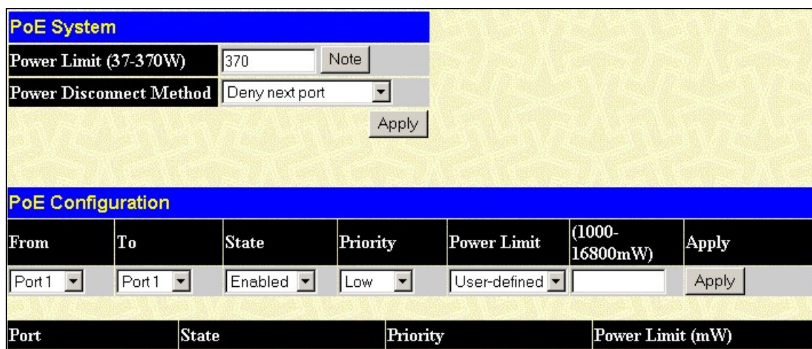
Figure 6- 6. PoE Configuration window
