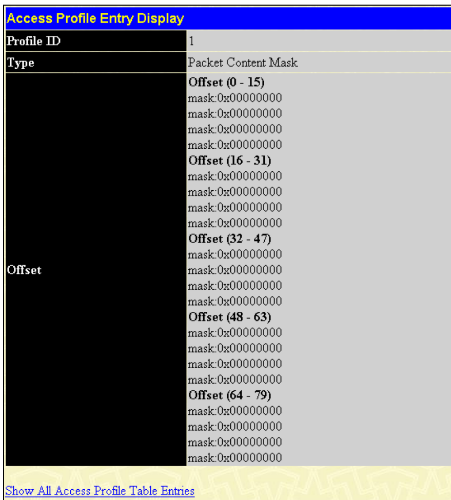
Figure 10- 7. Access Profile Entry Display window (Packet Content Mask)
