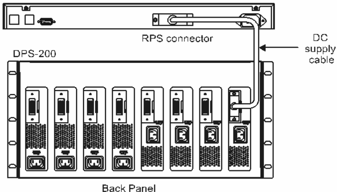
Figure 2 - 10. The DES-3828 with the DPS-200 chassis RPS
