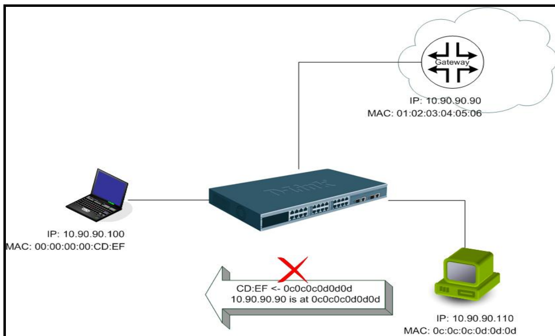
Example Topology
