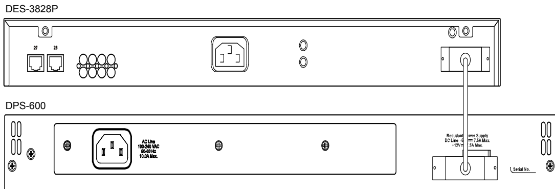
Figure 2 - 11. DES-3828P with the DPS-600 External Redundant Power Supply
