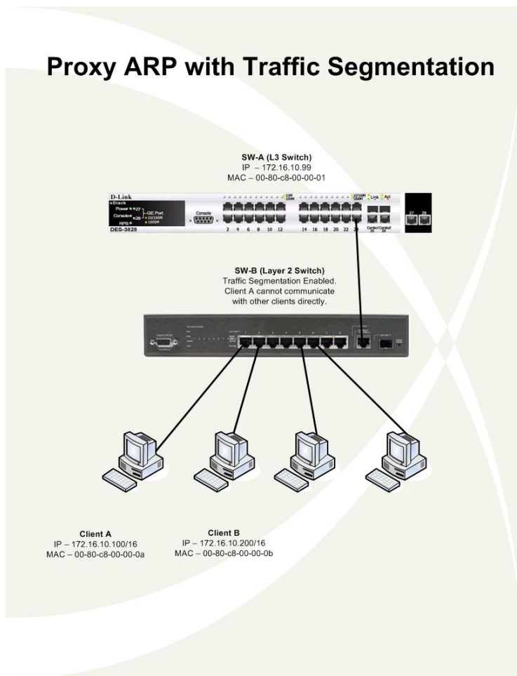
Figure 8- 1. Proxy ARP with Traffic Segmentation
