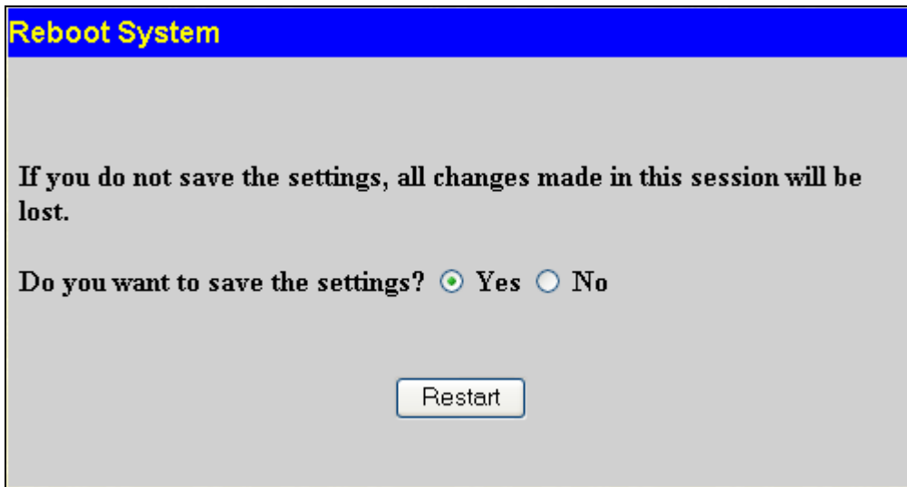
Figure 13- 2. Reboot window
