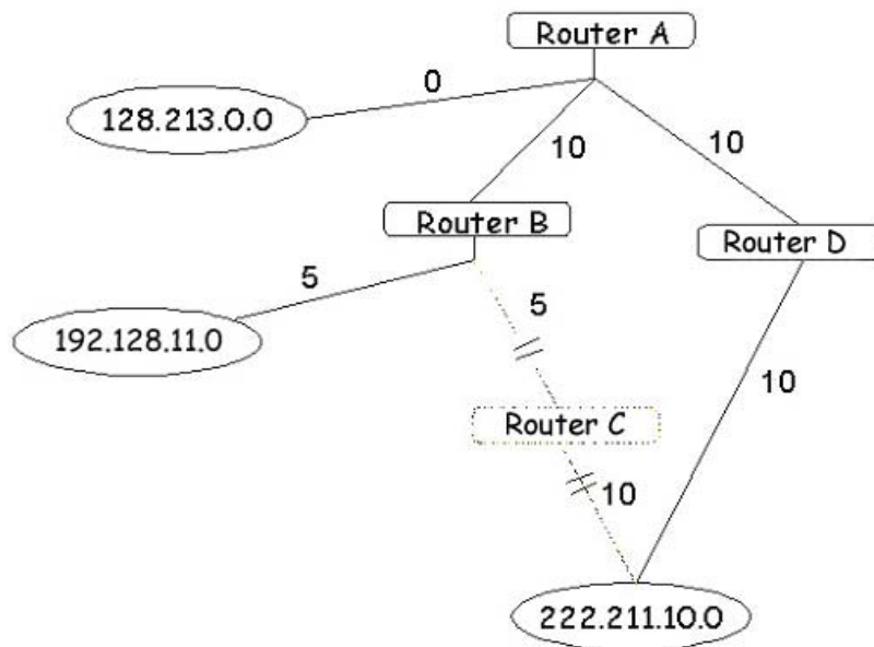
Figure 8- 17. Constructing a Shortest Path Tree
